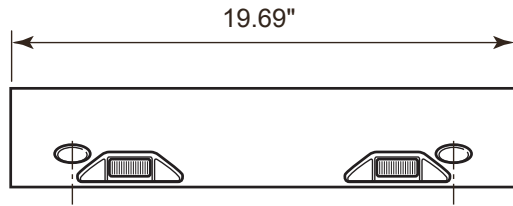
Front Elevation (Inner Section)
