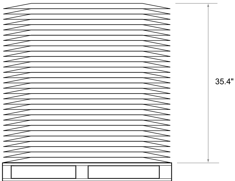
30 SAFE COVERS ON PALLET
