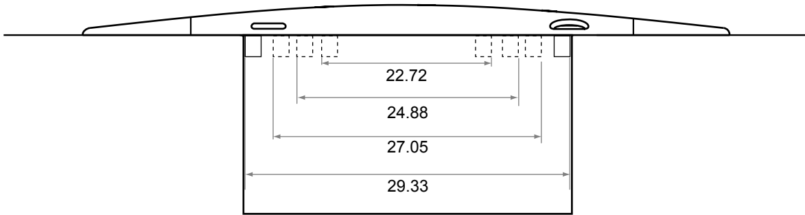
IN USE ON TRENCH SHOWING TRENCHPIN SYSTEM
