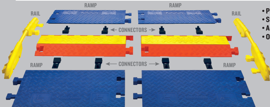
System shown with 2 Heavy Duty Linebackers, 2 Pairs of Ramps and 8 Connectors. Ramps available only in blue and rails available only in yellow.
